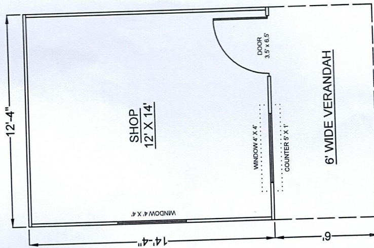
LAYOUT PLAN
